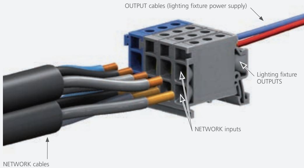
Example: assembly of 4 BD2 terminals to connect 2 network cables (4 conductors)
